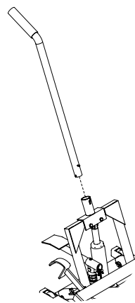
Figure 8: Handle assembly.
