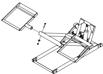
Figure 5: Wheel Basket attachment.
