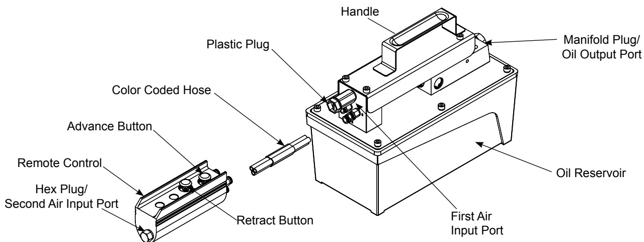
Figure 1 - Model PA1500L & PA3801L Components (PA1500L shown)
