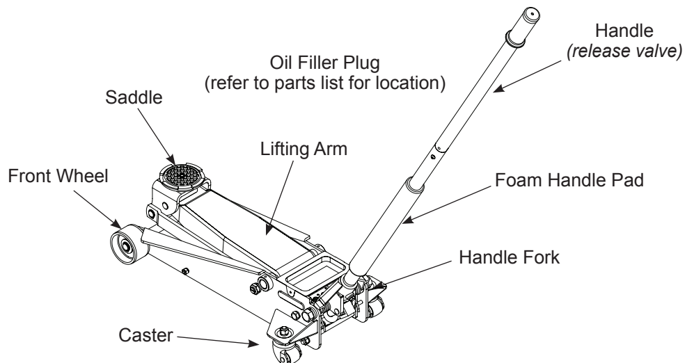
Figure 1 - Typical Jack Nomenclature
