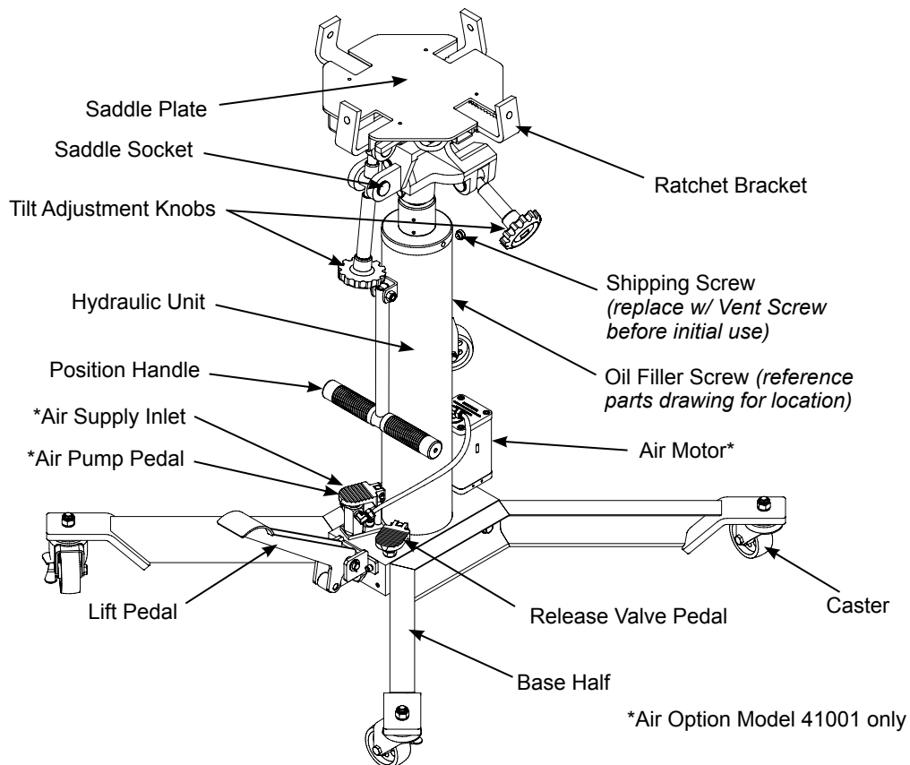
Figure 1- Typical Transmission Jack Components (41001 shown)
