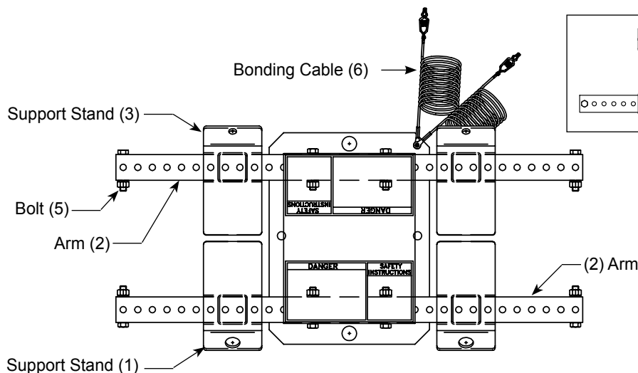
Figure 5 - Assembly instruction
