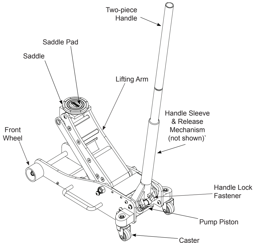
Figure 1 - Service Jack Nomenclature
