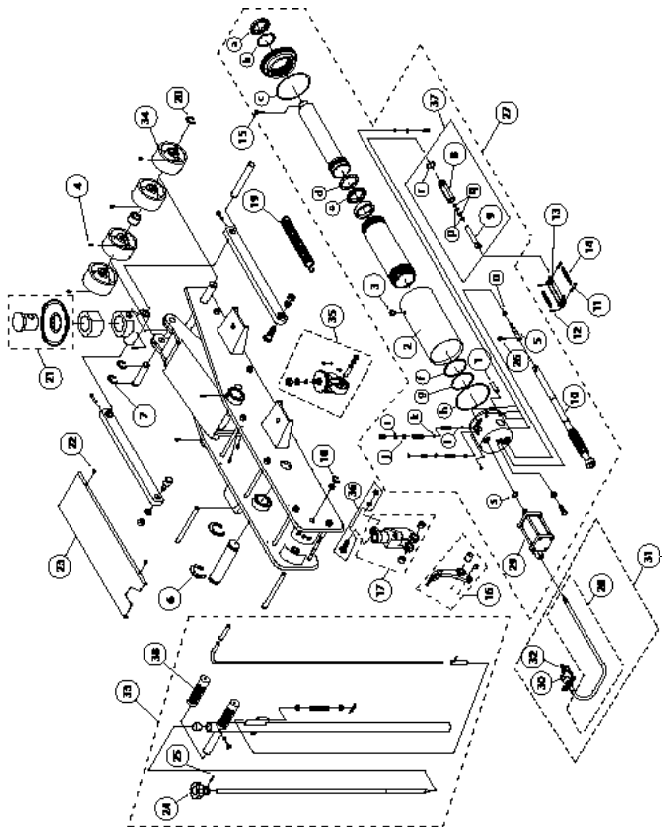
Figure 3 - Replacement Parts Illustration for Model 22203
